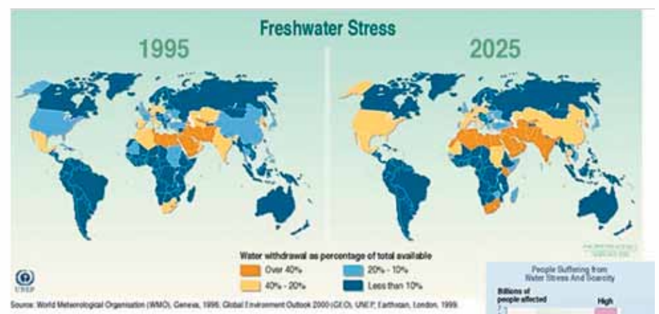
Fig. 1: World Meteorological Organization forecasts freshwater stress in the year 2025.
